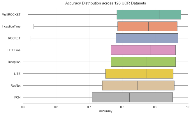
Fig. 6. Accuracy distribution across univariate datasets demonstrating performance consistency across configurations.
