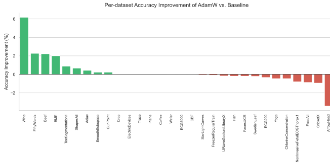
Fig. 3. Dataset-level improvement comparison demonstrating performance gains from optimization strategies including AdamW and differenced input channels.
