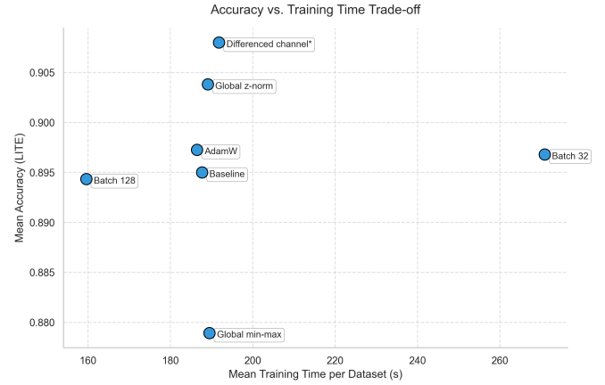
Fig. 4. Training time versus accuracy comparison across configurations. Efficient configurations achieved improved performance without significant runtime increase.
