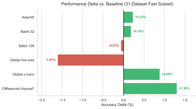
Fig. 2. Mean accuracy comparison across different configurations. Batch size 32 achieved slightly higher accuracy than the baseline, while batch size 128 resulted in a small accuracy reduction.
