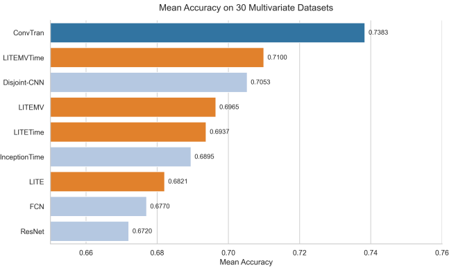
Fig. 8. Performance comparison across multivariate time series classification models.
